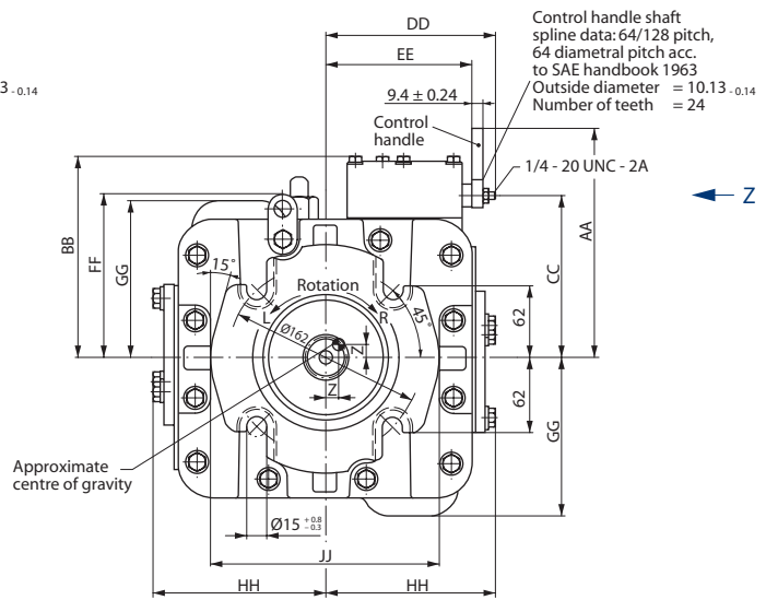
View X (for SPV 2/033 - 2/052 only)
