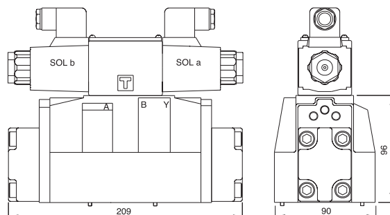
Front & Side View - Mainstage and Pilot 4WE16...53/.....NZ4
