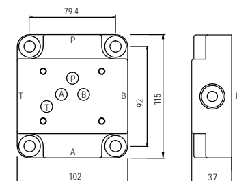
Top & Side Views - G67/01-SE
