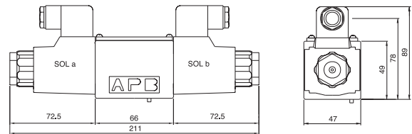
Front & Side View - 110 / 240 Volt AC 4WE6...75/AC...NZ4 Series
