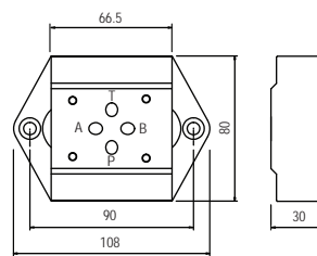
Top & Side Views - G67/01
