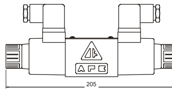
Front & Side View - 110 / 240 Volt AC DFA-02-...-AC...-L-35 Series
