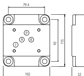
Top & Side Views - G67/01
