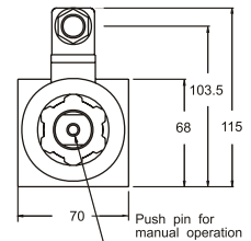
End View - DC & AC
