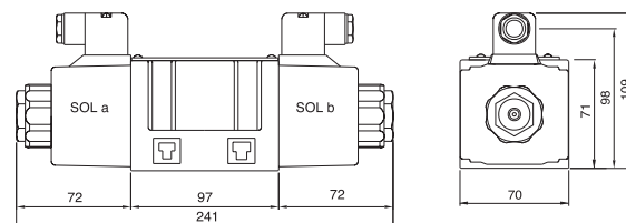
Front & Side View - 110 / 240 Volt AC 4WE10...23/AC...NZ4 Series
