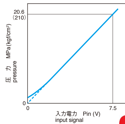
◆ 電圧-圧力特性 Voltage-pressure rated characteristics
