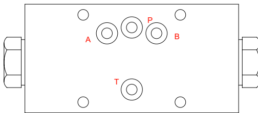
Pilot Operated Check Module
