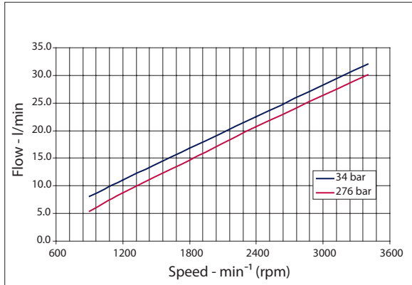
Model 10D (l/min)
