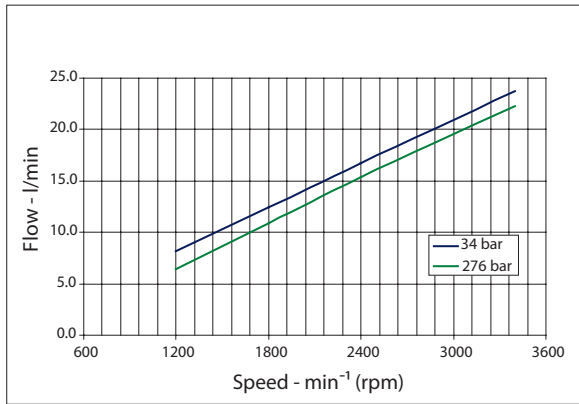
Model 07D (l/min)
